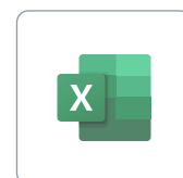
MICROSOFT EXCEL
